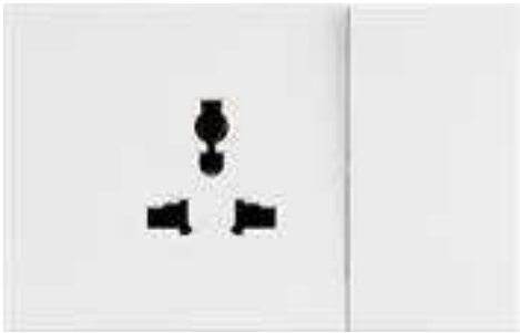
HK7210 10A / 120-250V 16A / 120-250V HK7210.3W 10A / 120-250V 16A / 120-250V
